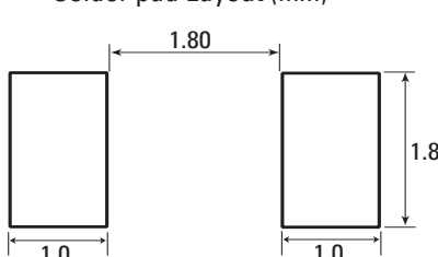
Solder pad Layout (mm)
