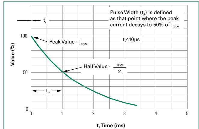
Figure 2. 10/1000 \mu s Pulse Waveform
