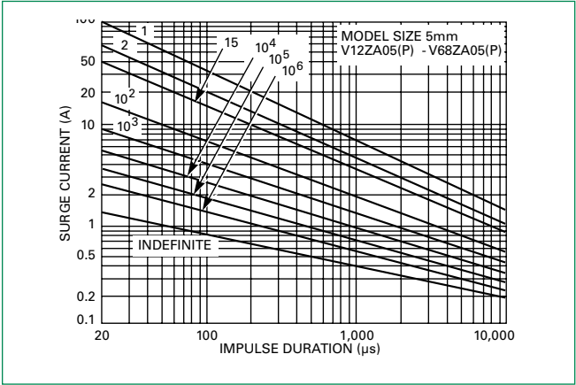
Figure 14 - V18ZA05(P) - V68ZA05(P)
