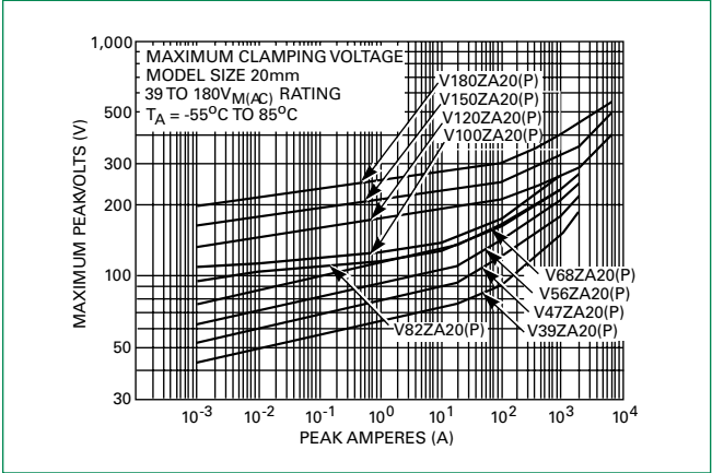
Figure 12 - V39ZA20(P) - V180ZA20(P)
