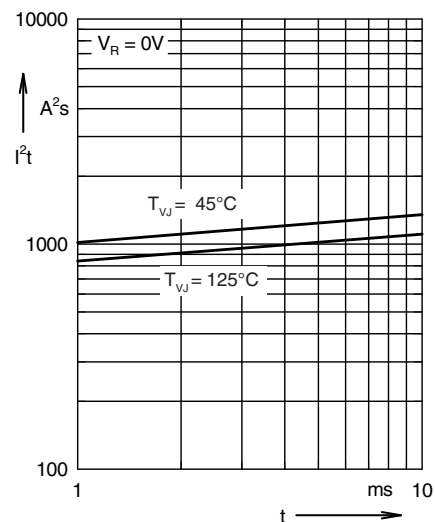
Fig. 8 I^2t vs, time (per thyristor)
