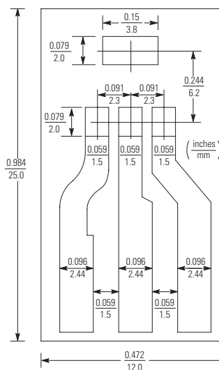
Figure 1. PCB for Thermal Impedance and Power Testing of SOT-223
