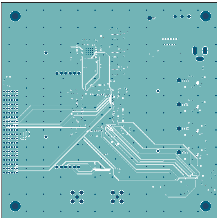
FIGURE A-25: ADM00825 – BOTTOM COPPER
