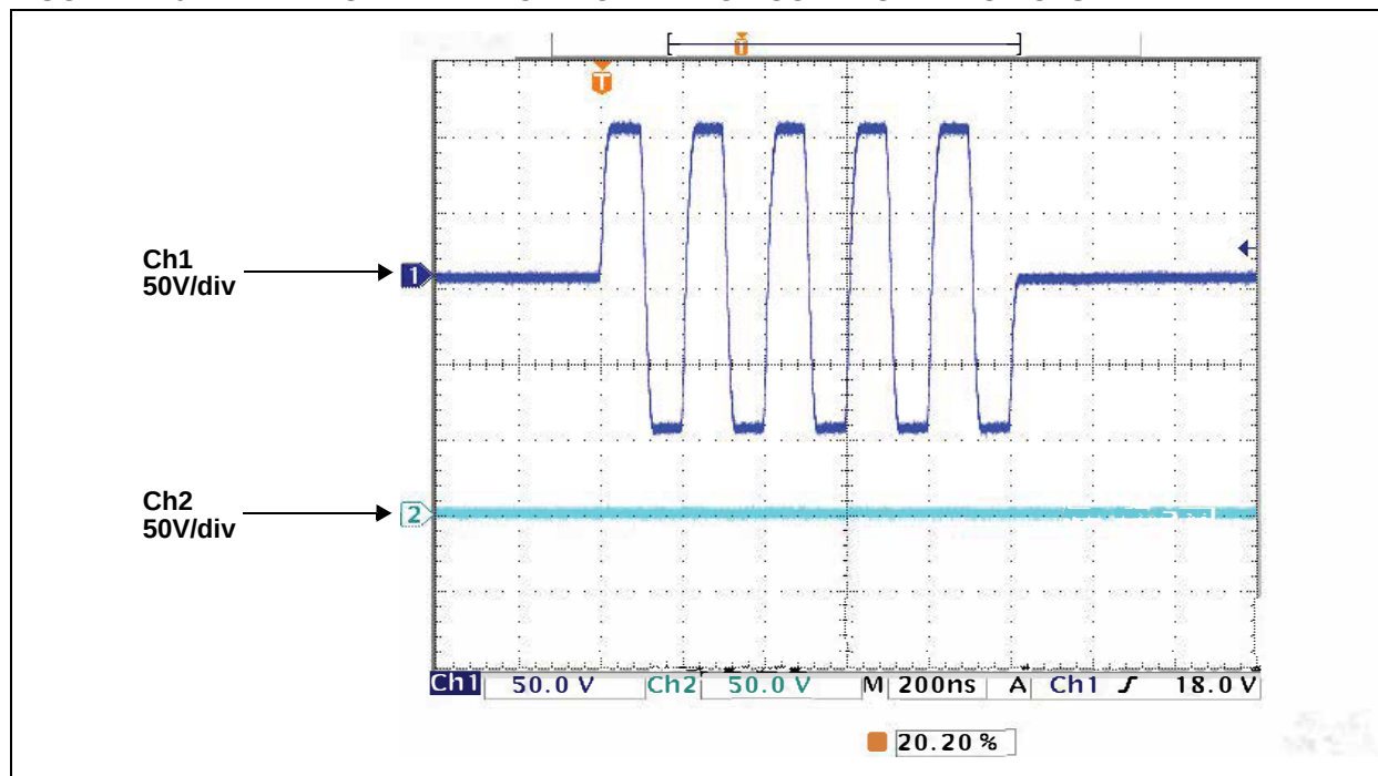
FIGURE 2-10: TYPICAL WAVEFORM OF 2:1 MUX CONNECTED TO PULSER
