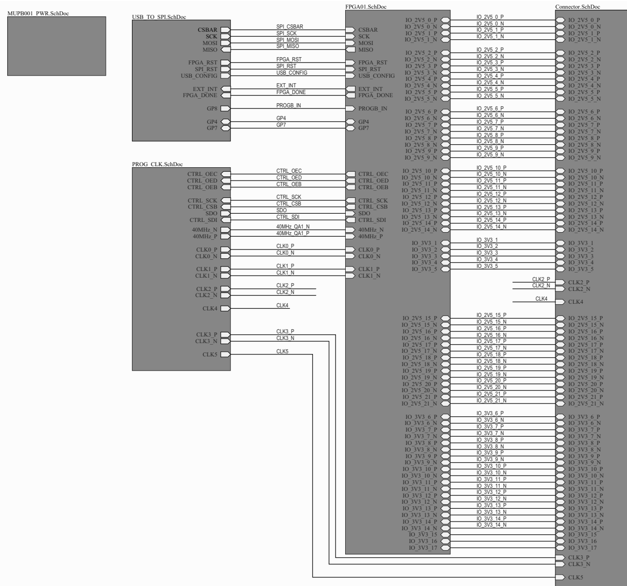
FIGURE A-11: ADM00825 – SCHEMATIC (CONNECTION)
