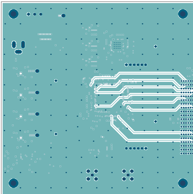
FIGURE A-24: ADM00825 – INNER 4
