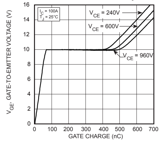
FIGURE 4, Gate charge
