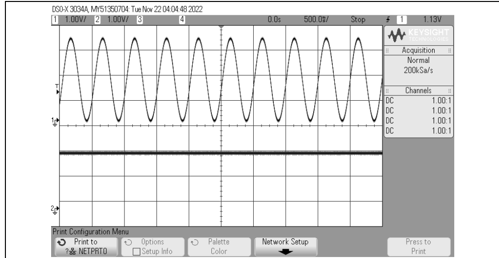
FIGURE 2-15: SPI Output Sine Wave (LED D4 Blinking, LEDs D2, D3 and D5 OFF, Channel 1 - SPI, Channel 2 - I^2C ).
