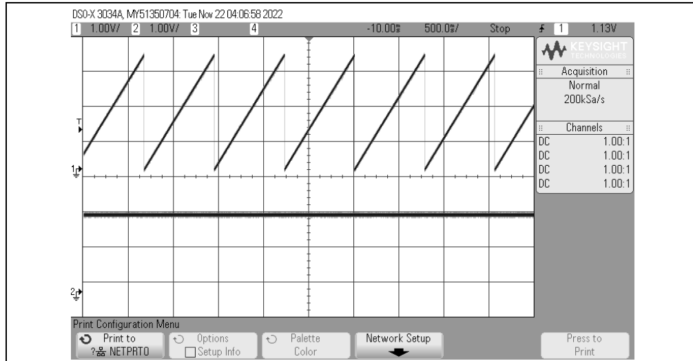
FIGURE 2-17: SPI Output Saw-Tooth Waveform (S1 Switch Pressed, LED D5 Blinking, LEDs D2, D3 and D4 OFF, Channel 1 - SPI, Channel 2 - I^2C ).
