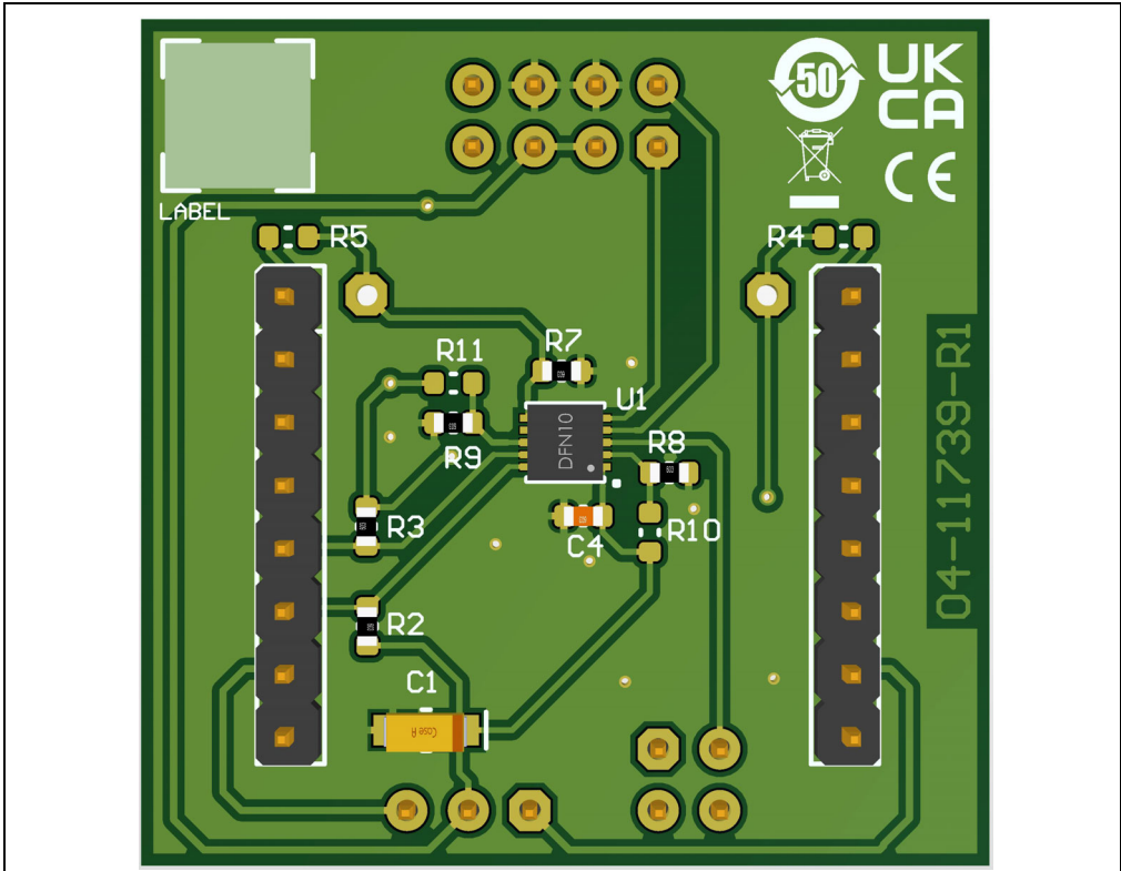
FIGURE 1-2: 1LSb INL Dual DAC Evaluation Board (Bottom View).
