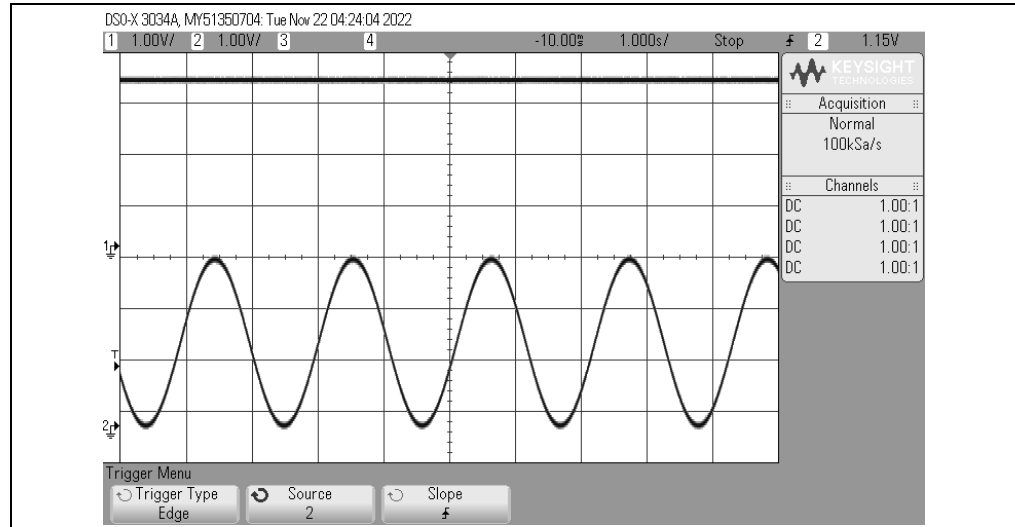
FIGURE 2-19: I 2 C Output Sine Wave (LED D2 blinking, LEDs D3, D4 and D5 OFF, Channel 1 - SPI, Channel 2 - I 2 C).
