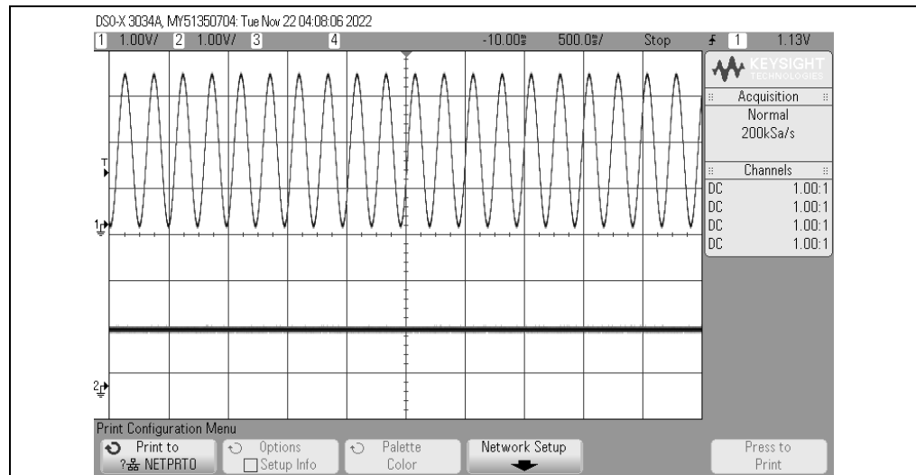
FIGURE 2-16: SPI Output Sine Wave with Varying Frequency using the Potentiometer (LED D4 Blinking, LEDs D2, D3 and D5 OFF, Channel 1 - SPI, Channel 2 - I^2C ).
