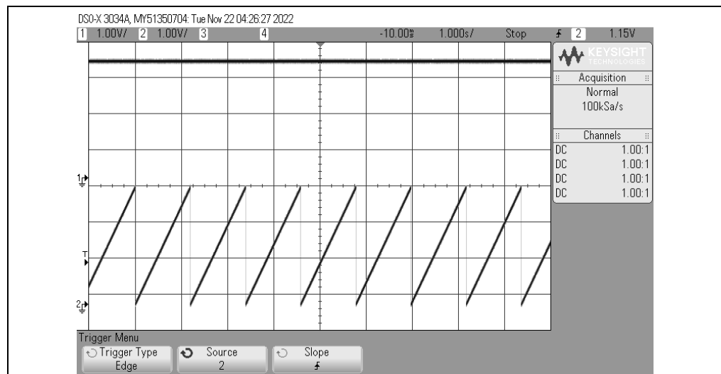
FIGURE 2-20: I 2 C Output Saw-Tooth Waveform (LED D3 blinking, LEDs D2, D4 and D5 OFF, Channel 1 - SPI, Channel 2 - I 2 C).
