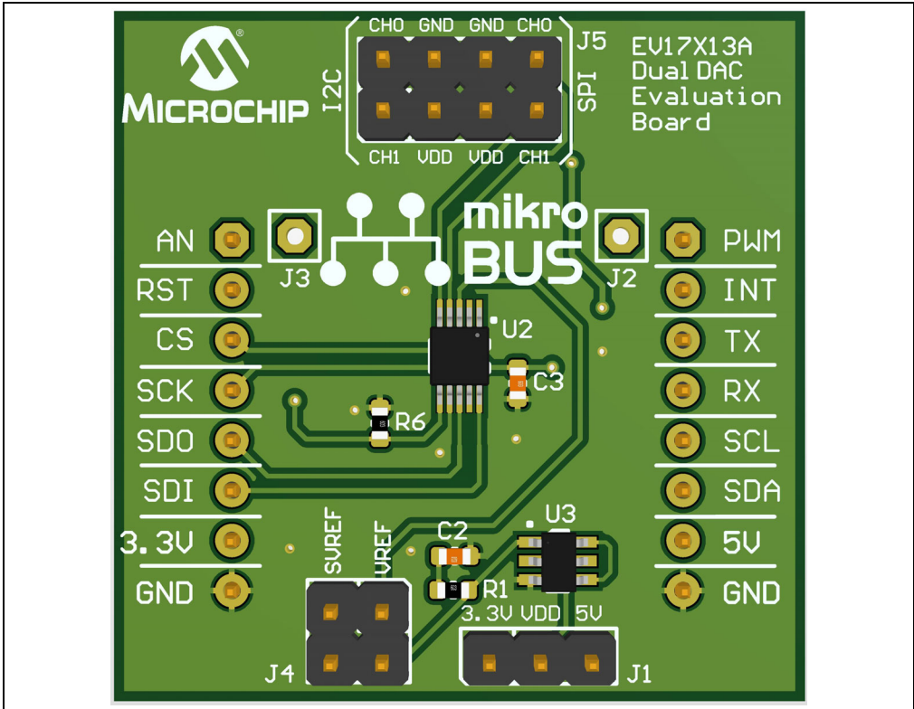
FIGURE 1-1: 1LSb INL Dual DAC Evaluation Board (Top View).
