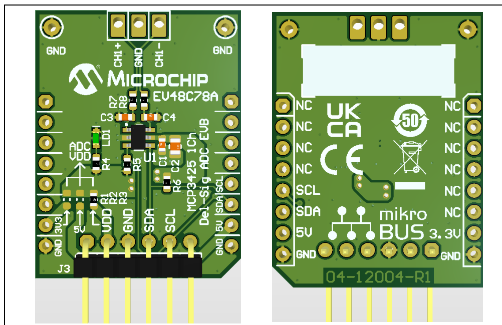
FIGURE 1-3: Top and Bottom Views of the MCP3425 Evaluation Board (EV48C78A).
