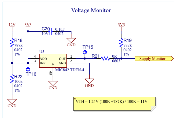
Figure 3-11. Voltage Monitoring Schematic
