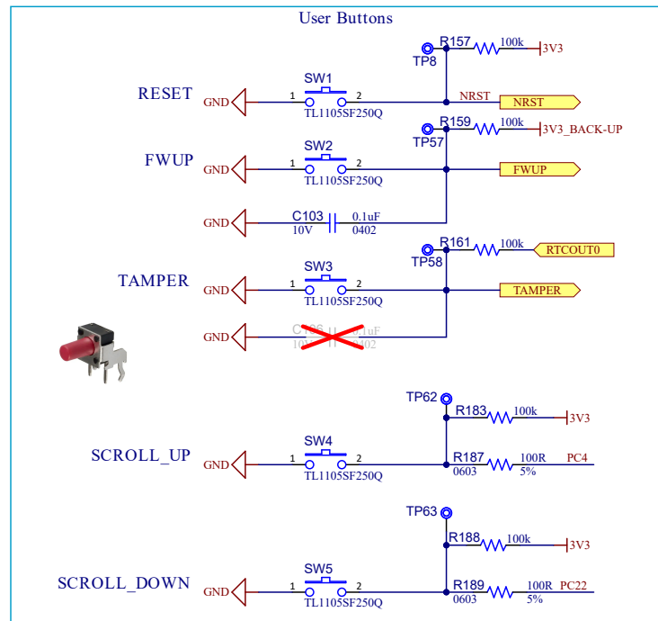
Figure 3-29. Buttons Schematic
