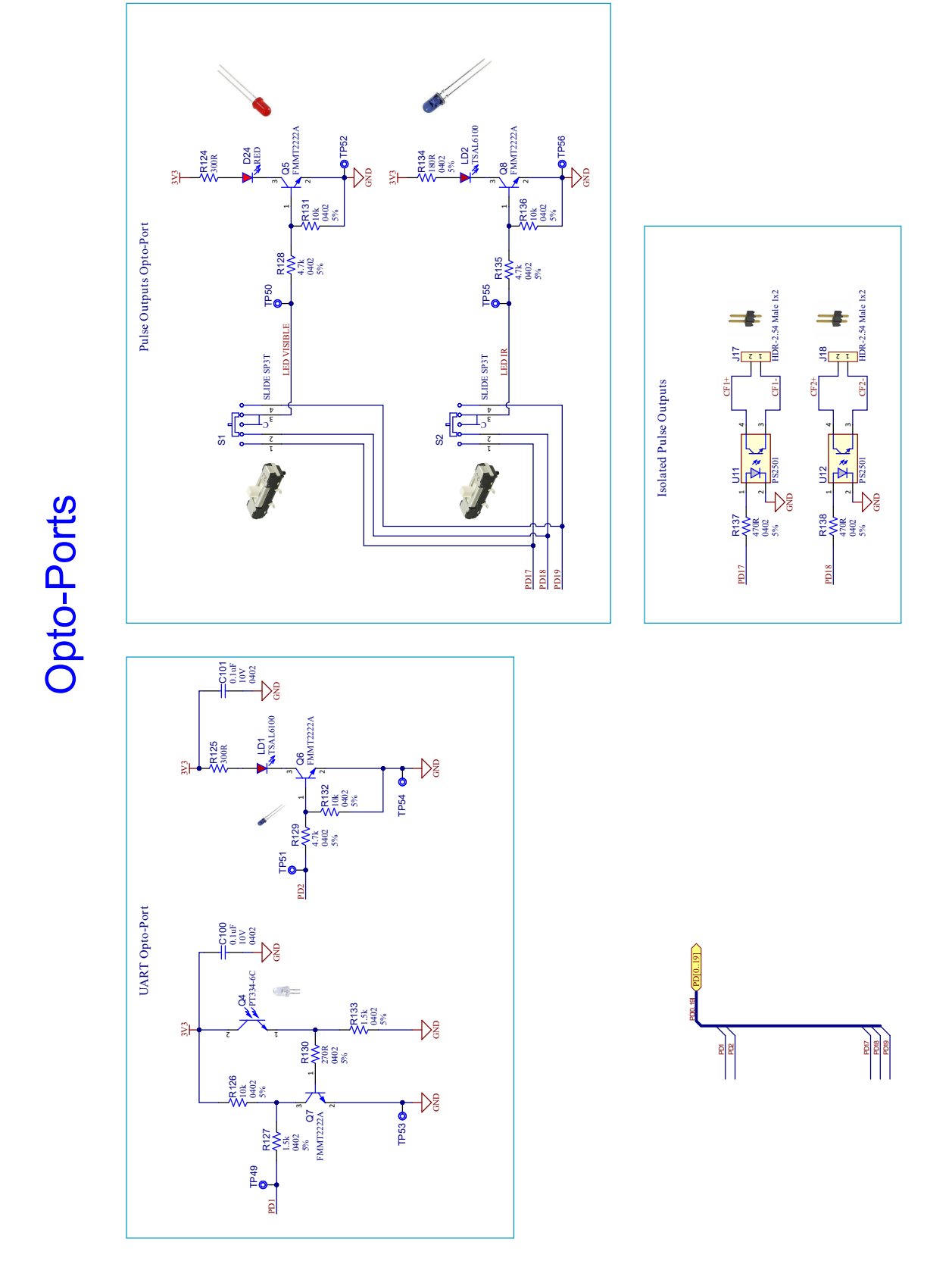
Figure 5-8. Opto-Ports Schematic
