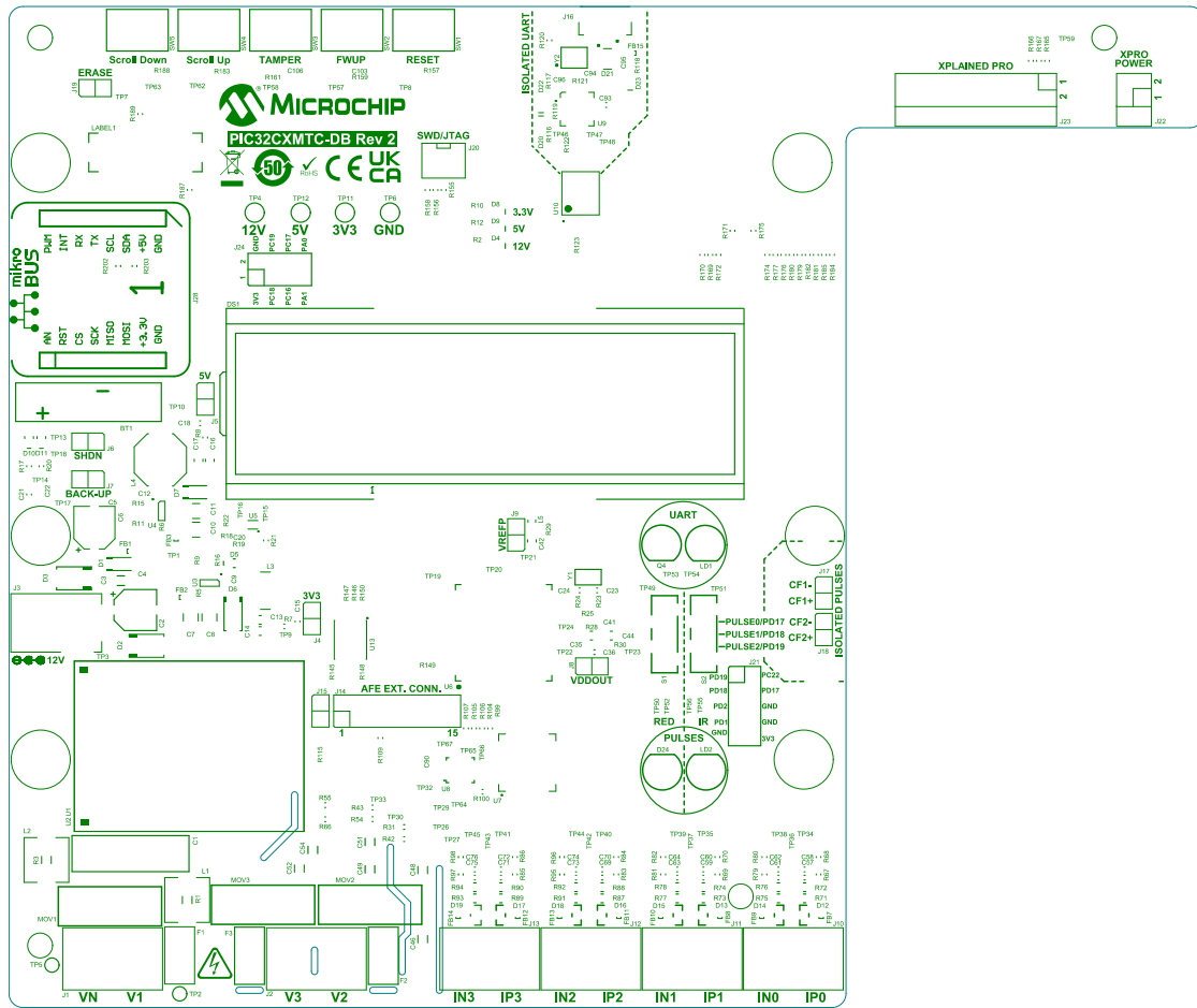
Figure 5-14. PIC32CXMTc-DB Layout: Top Silkscreen
