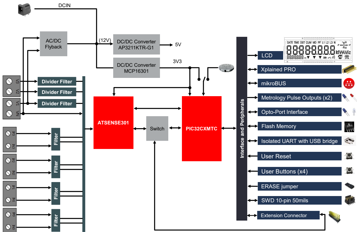
Figure 3-2. PIC32CXMT-DB Block Diagram
