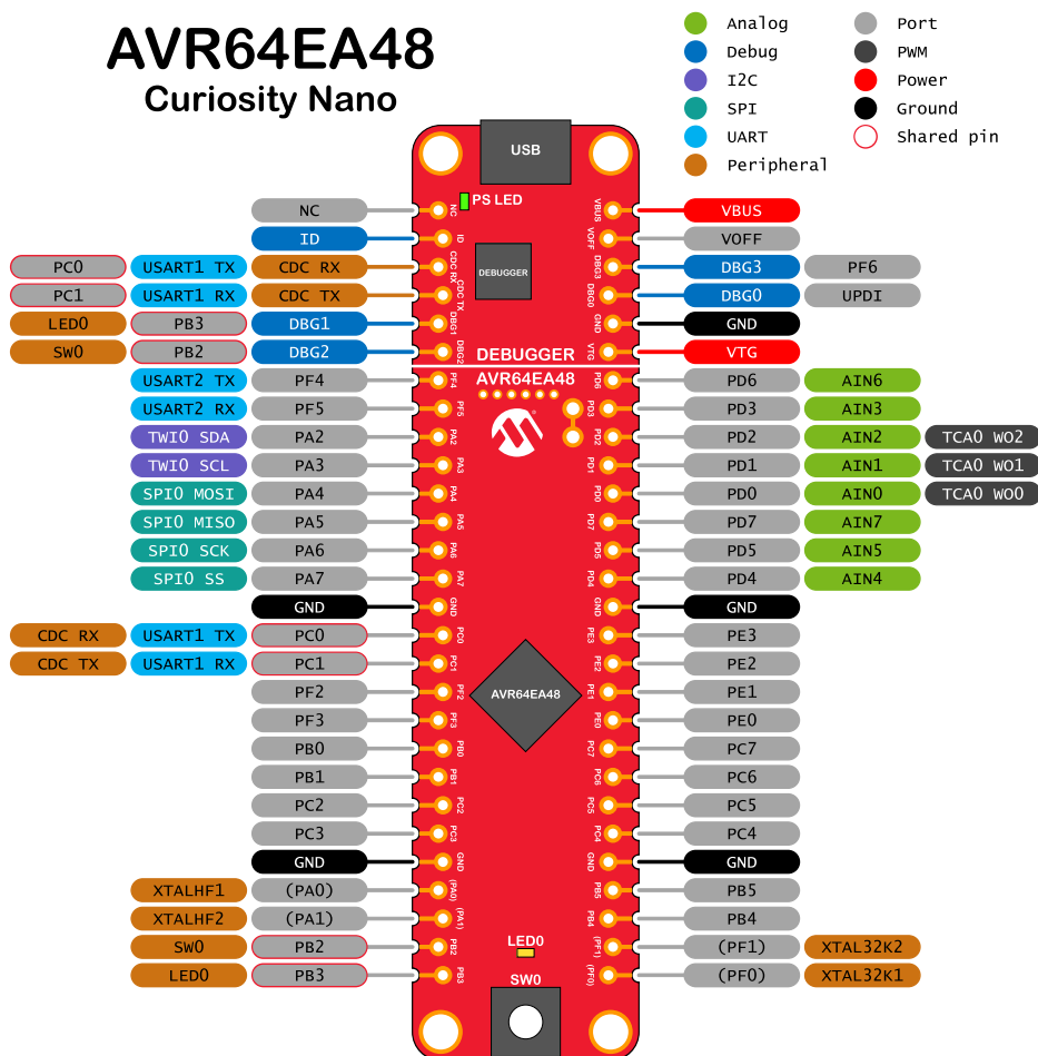
Figure 4-1. AVR64EA48 Curiosity Nano Pinout
