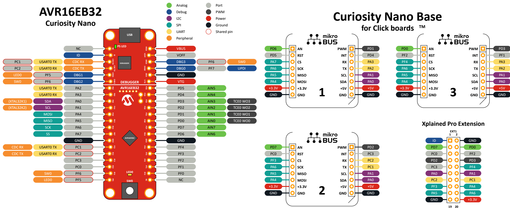
Figure 6-5. AVR16EB32 Curiosity Nano Pinout Mapping
