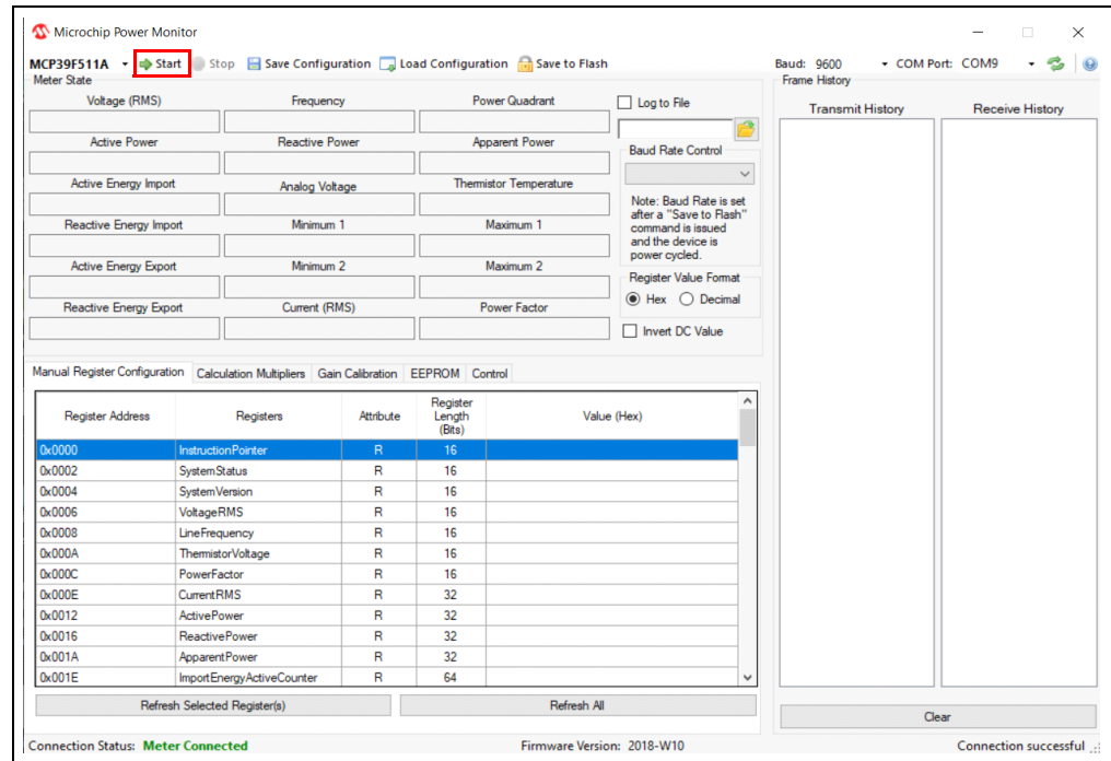
FIGURE 2-4: DATA ACQUISITION
