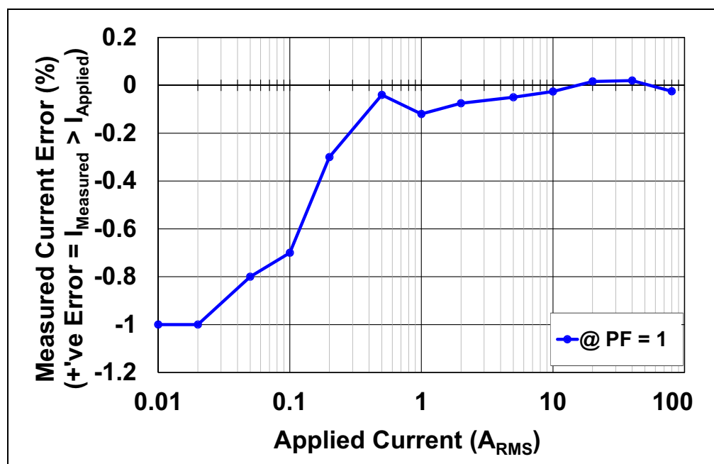
FIGURE 4-1: Current Measurement Error (%).
