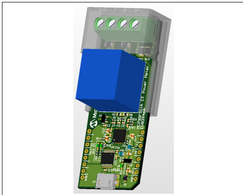
FIGURE 1-1: MCP39F511A CT Power Meter.
