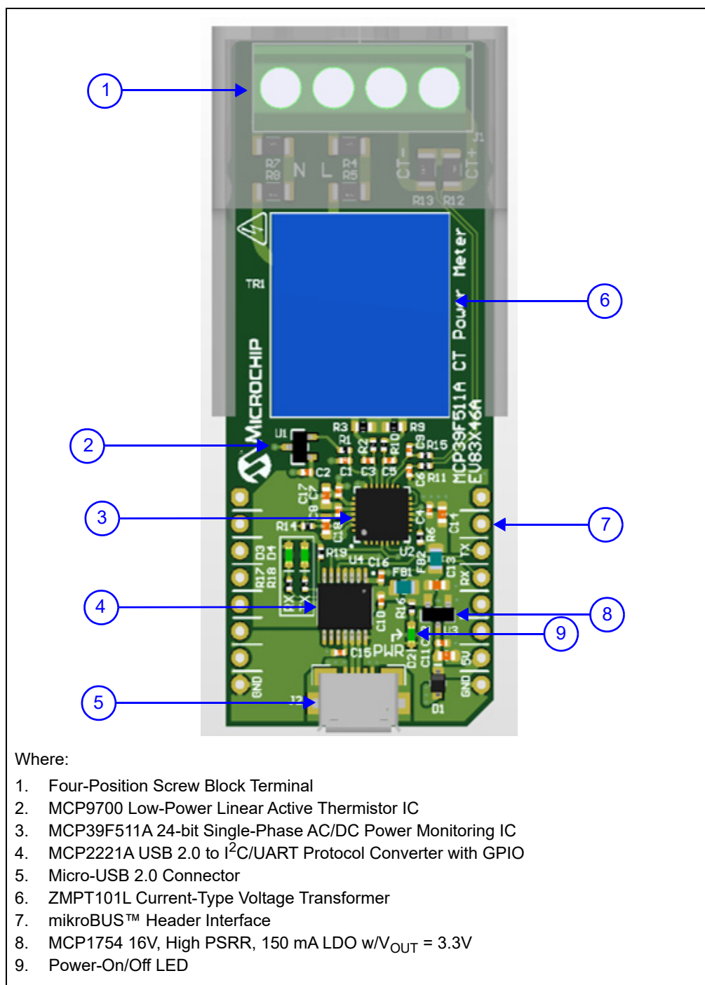
FIGURE 3-1: MCP39F511A CT Power Meter (Top View).
