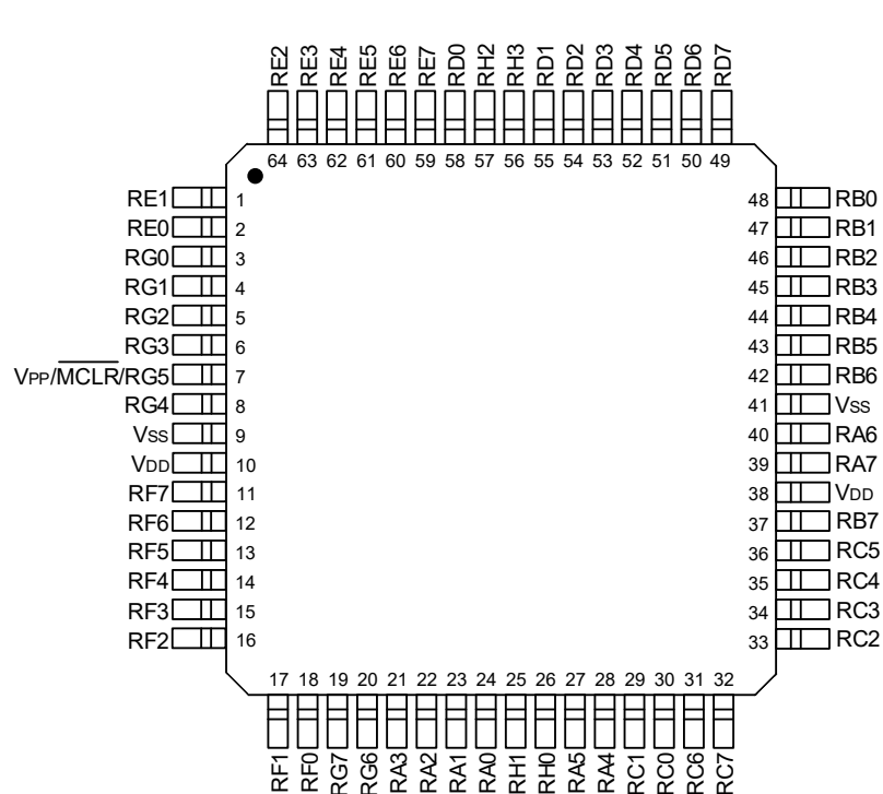
Figure 2-8. 64-Pin TQFP
