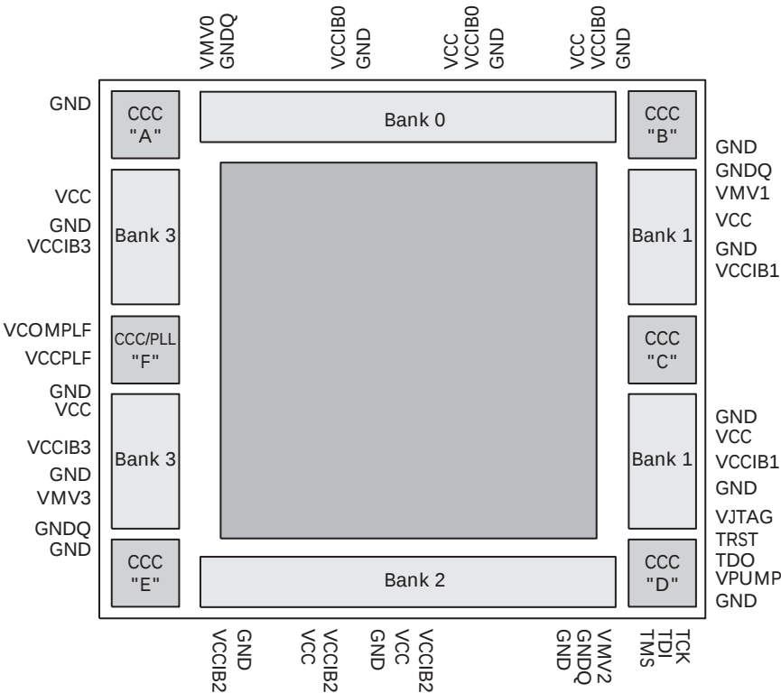
Figure 24 • M1AGL1000 Layout
