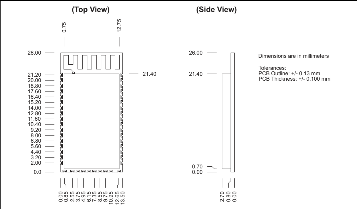
FIGURE 1-1: MODULE DIMENSIONS
