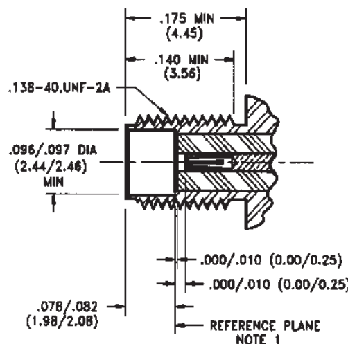
Female Jack
