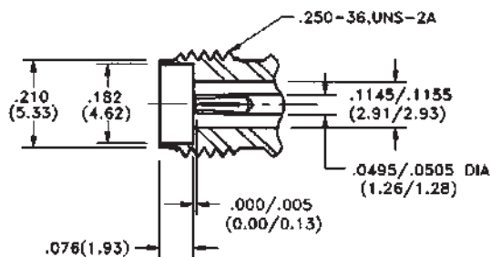
Female Jack
