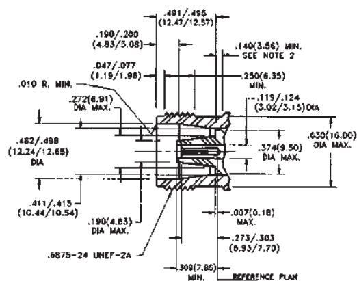
Female Jack
