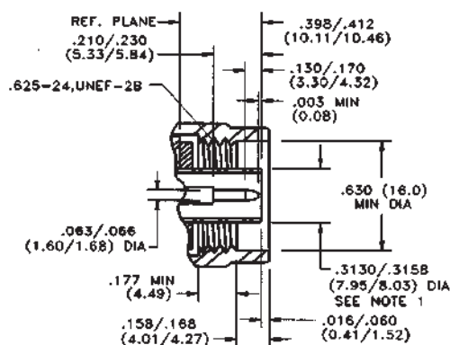
Male Plug
