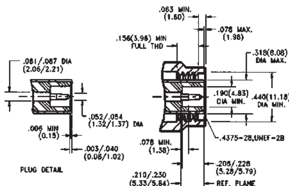
Male Plug
