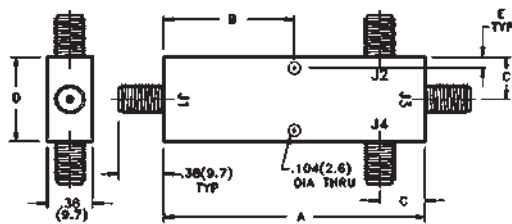
Case Style 2
