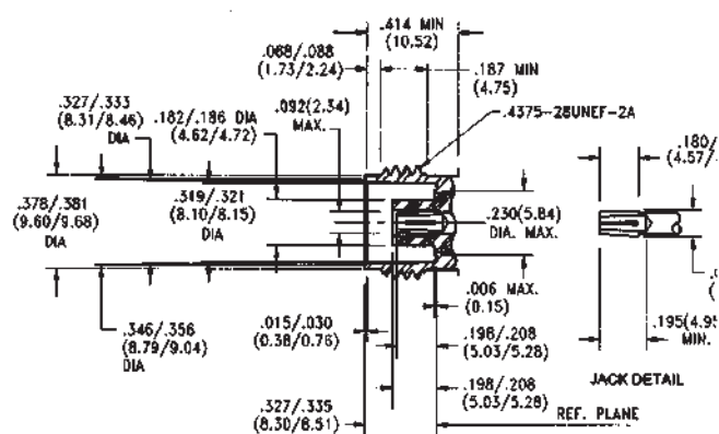
Female Jack
