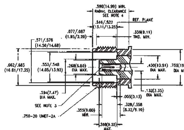
Female Jack
