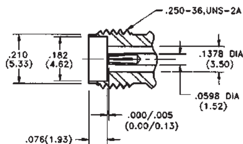
Female Jack
