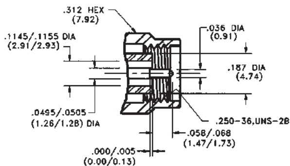
Male Plug
