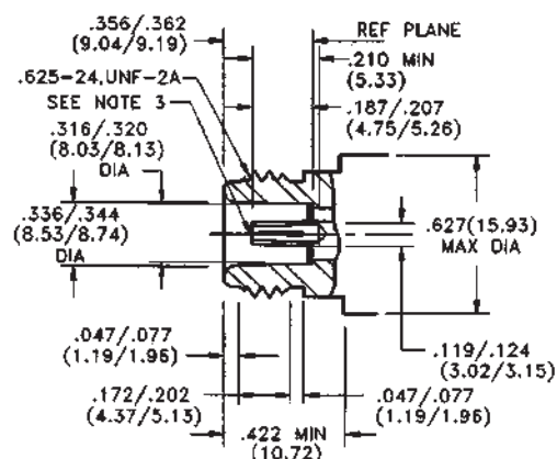
Female Jack
