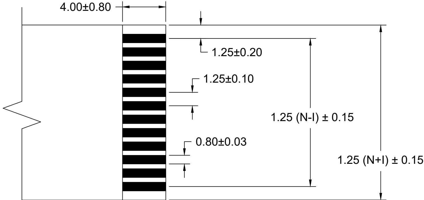
END TAIL DETAIL SCALE 5:1
