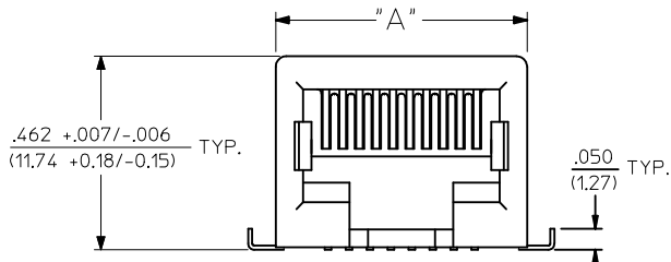
8 CIRCUIT ASSEMBLY
