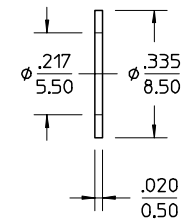
WASHER
