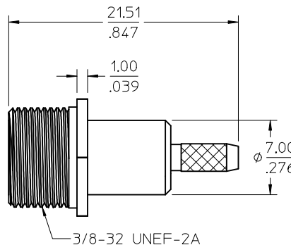
CABLE CONTACT
