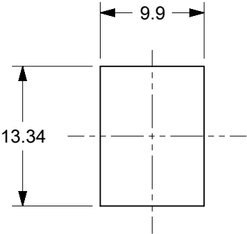
RECOMMENDED MOUNTING CUTOUT FOR 1.6mm THICK PANEL
