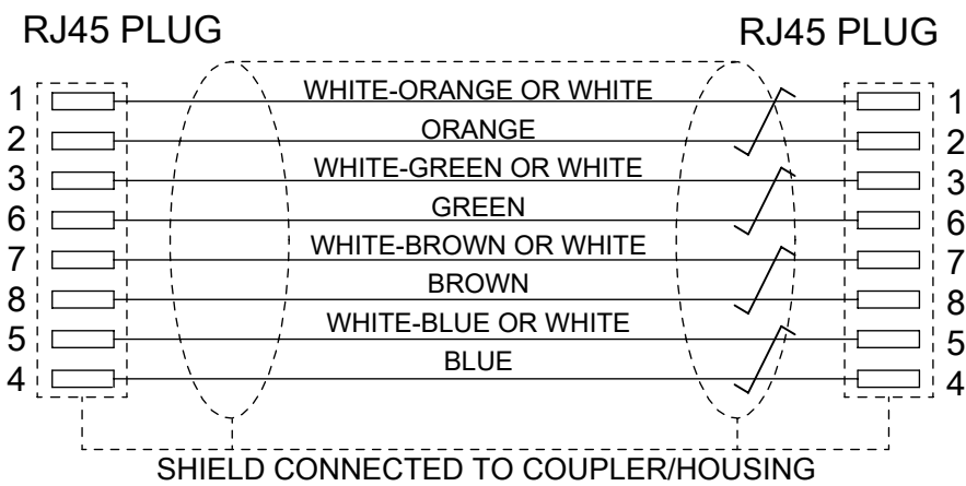
WIRING DIAGRAM
