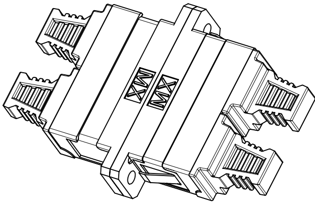
ISO VIEW 2 SCALE 1.5:1
