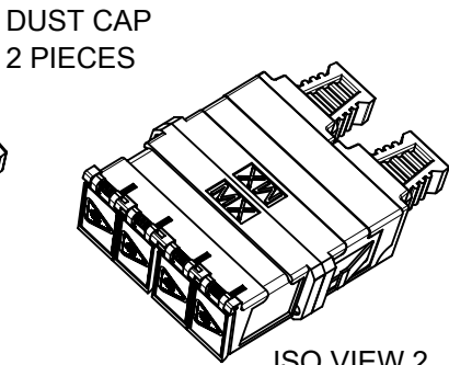
ISO VIEW 2 SCALE 1:1
