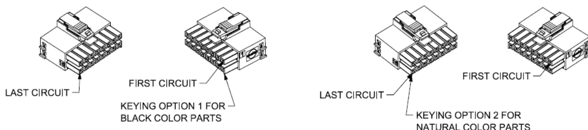
KEYING OPTION 1
