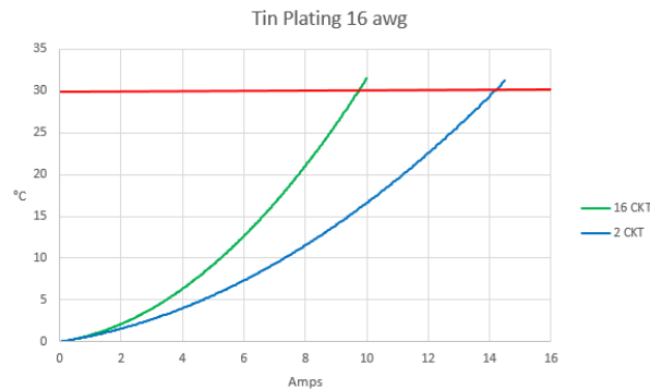
Temperature Rise vs. Current per EIA-364-70
