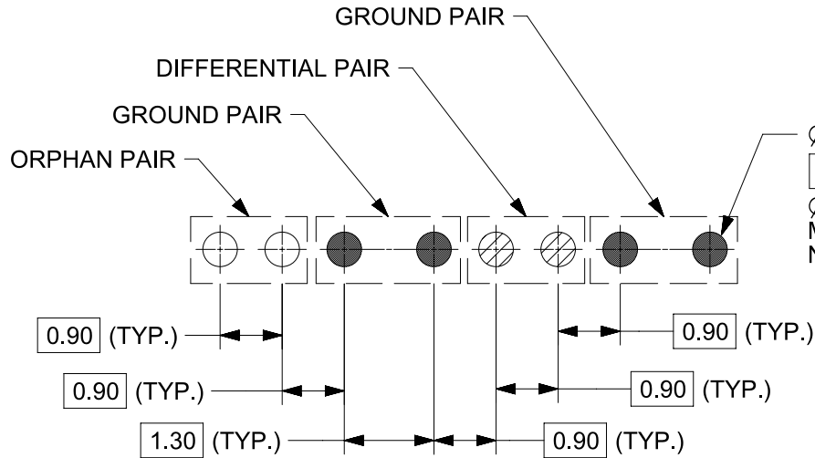
DETAIL A
