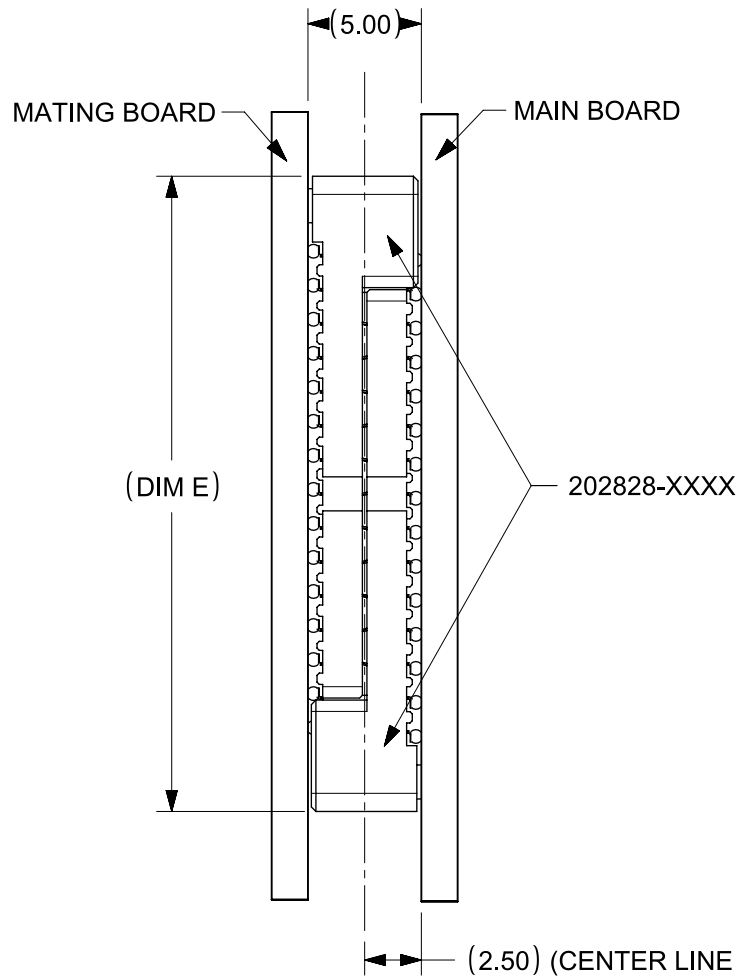
MATED DIMENSIONS
