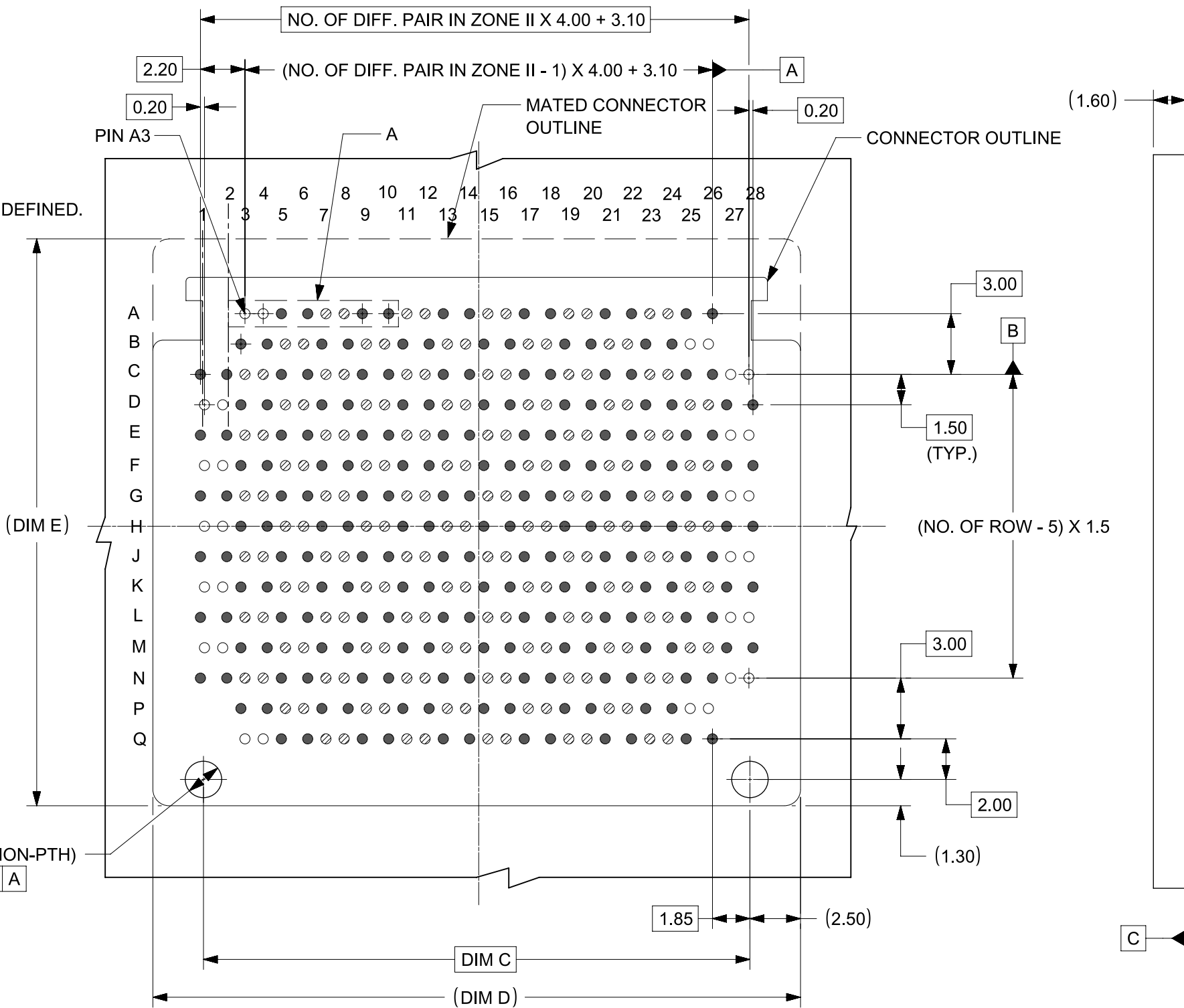
RECOMMENED PCB LAYOUT
