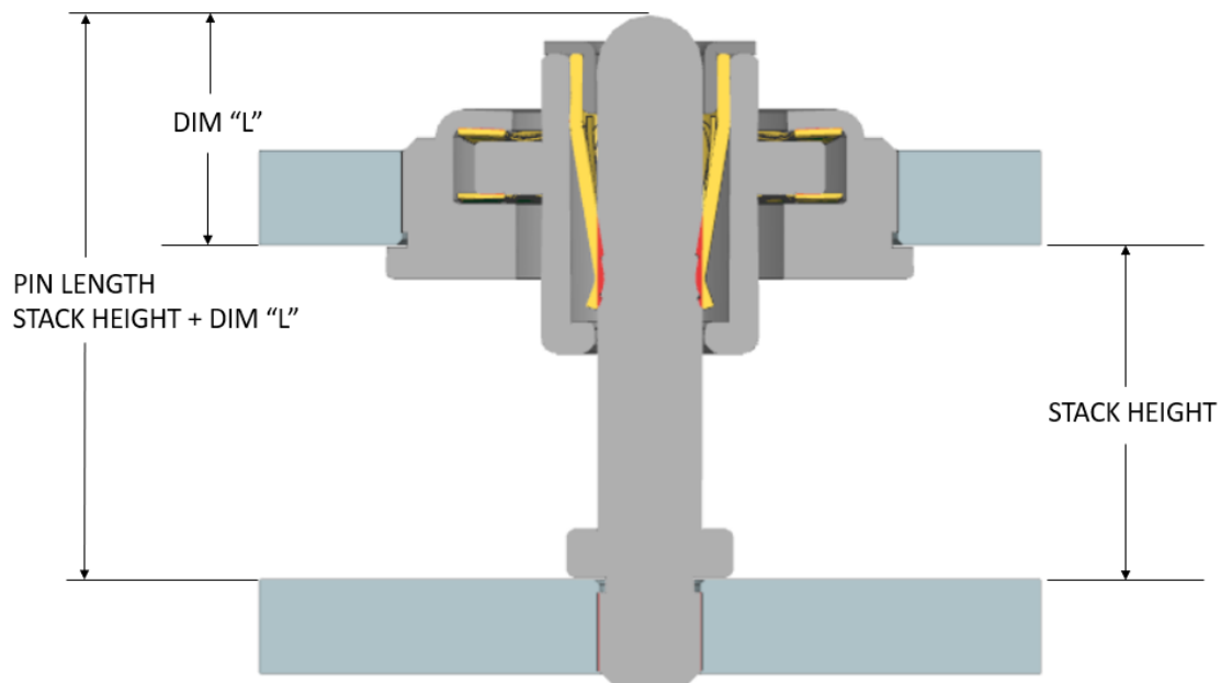
Figure 7.4.1 Press fit floater shown in view
