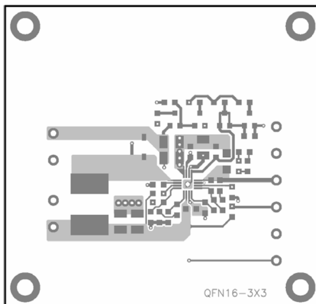
Figure 2: Top Layer
