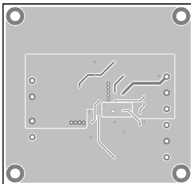
Figure 3: Bottom Layer
