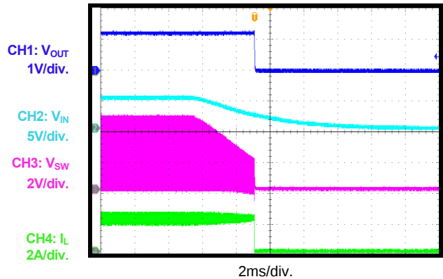
V_{IN} Shutdown
