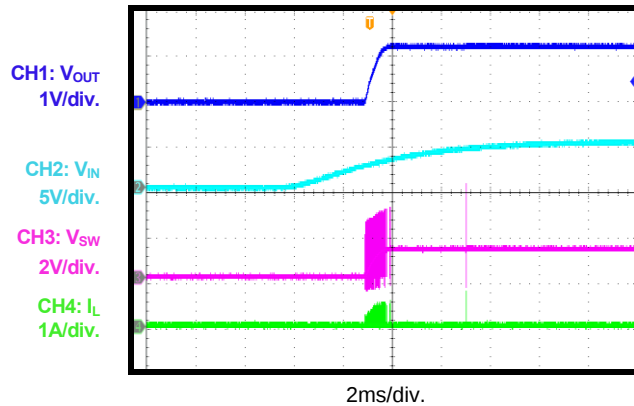
V_{IN} Power-Up
