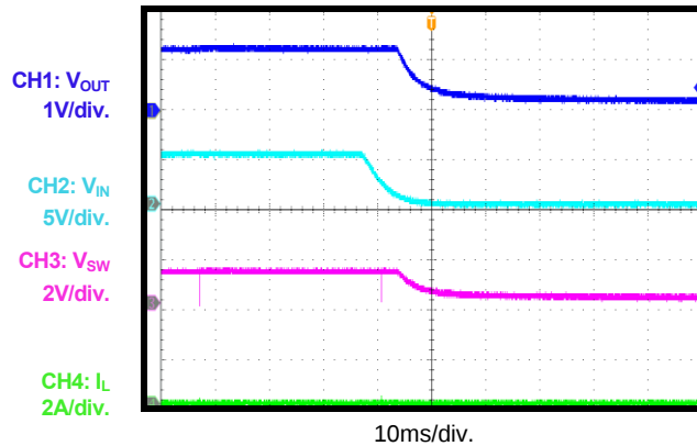
V_{IN} Shutdown
