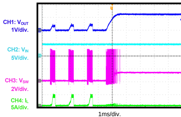
Short-Circuit Recovery
