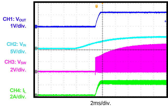
V_{IN} Power-Up
