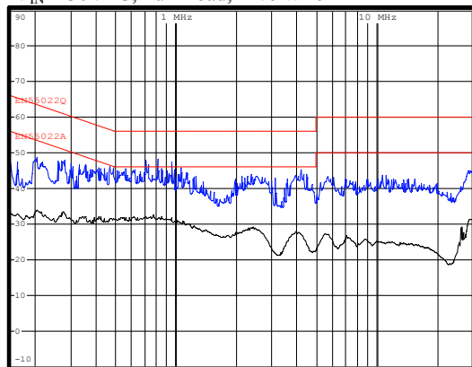
Conducted EMI
