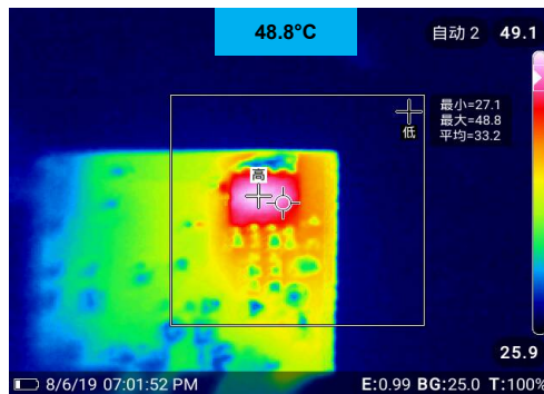
Thermal V_{IN}=265V_{AC}
