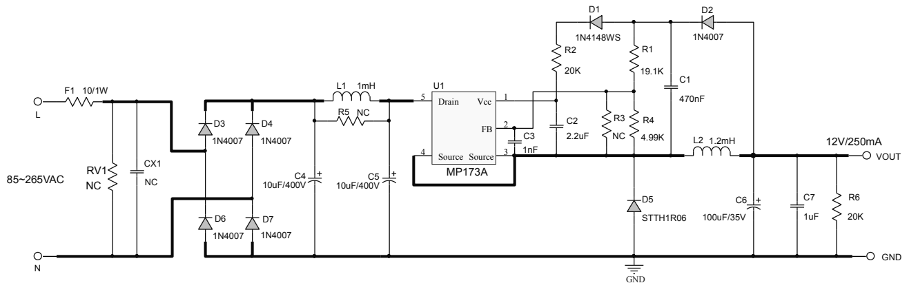
Figure 1: Schematic
