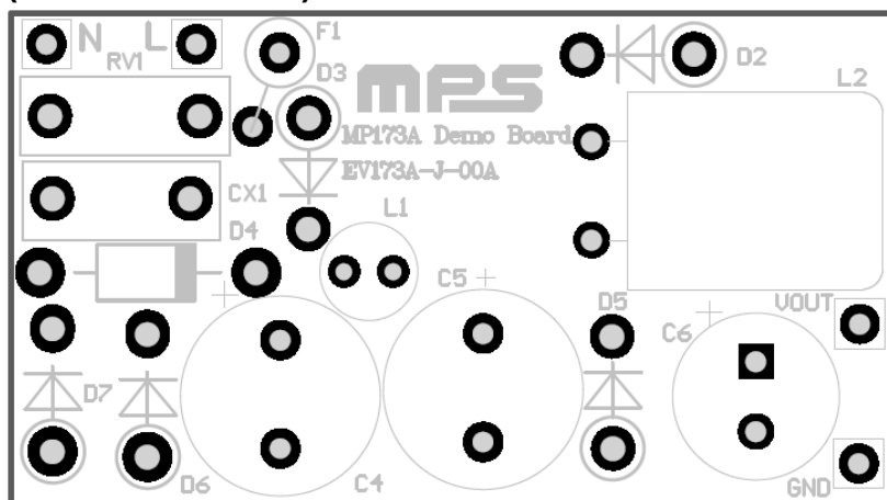
Figure 2: Top Layer
