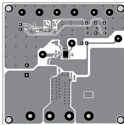
Figure 2: Top Layer
