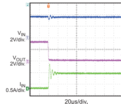
Short Output
