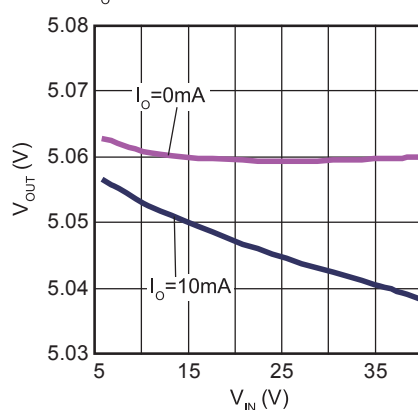
V_{OUT} vs. V_{IN} V_O = 5V
