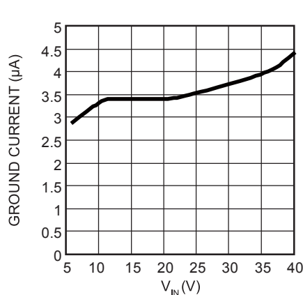
Ground Current vs. V_{IN} I_O = 0mA
