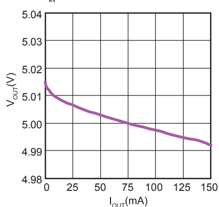
V_{OUT} vs. I_{OUT} V_{IN} = 6V
