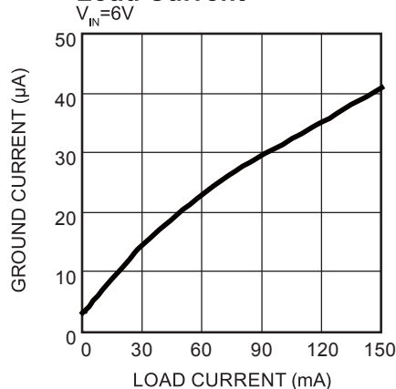
Ground Current vs. Load Current V_{IN} = 6V
