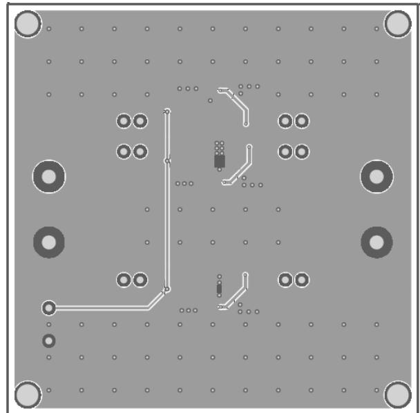
Figure 2 – Bottom Layer
