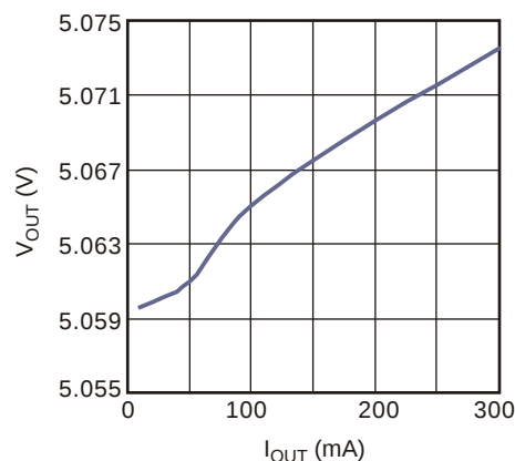
V OUT vs. I OUT V IN =6V
