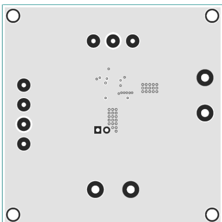
Figure 3—Inner 1 Layer
