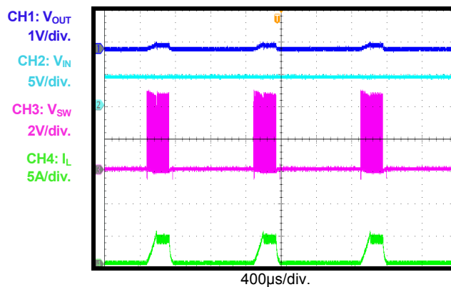
Short-Circuit State
