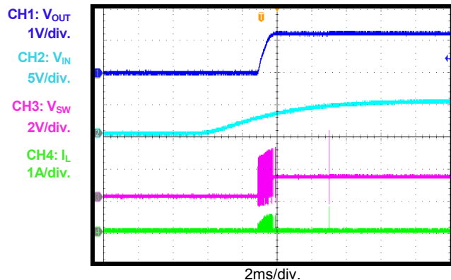
V_{IN} Power-Up
