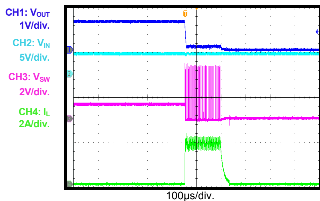
Short-Circuit Recovery
