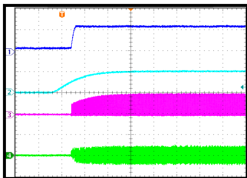
V_{IN} Power-Up
