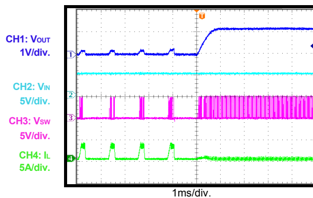
Short-Circuit Recovery
