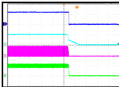
V_{IN} Shutdown
