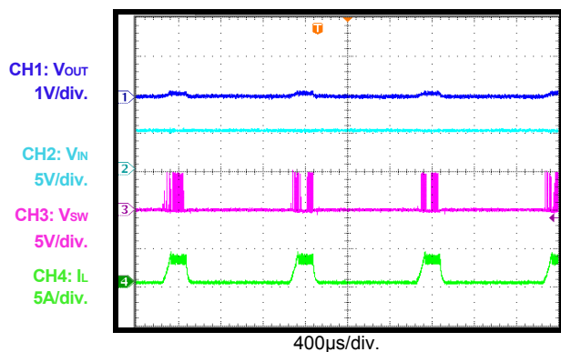
Short-Circuit State
