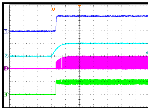
V_{IN} Power-Up
