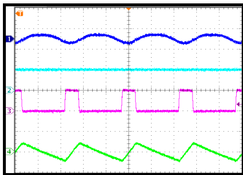
Steady State
