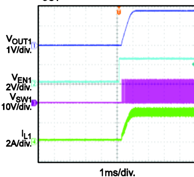
Startup through Enable (CH1)
