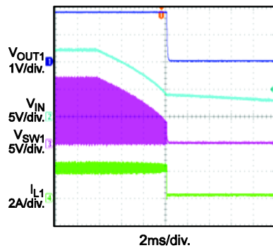
Shutdown through Input Voltage (CH1)
