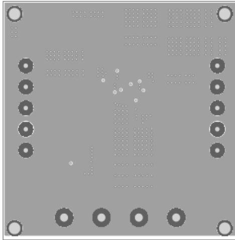
Figure 3—Inner1 Layer
