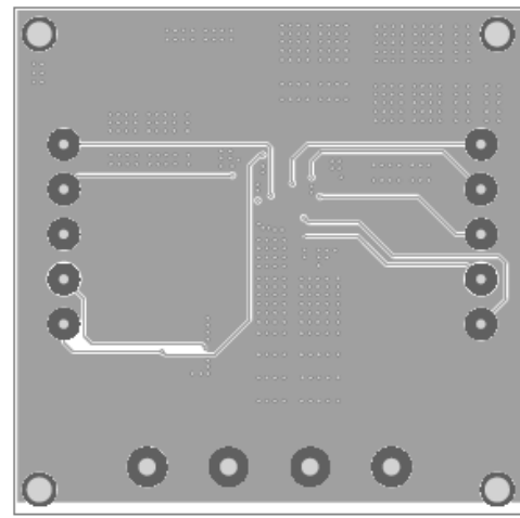
Figure 4—Inner2 Layer
