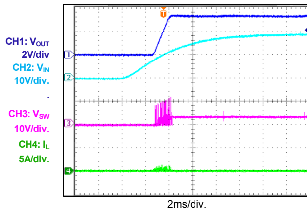
Startup through Input Voltage
