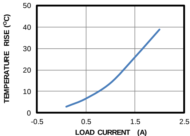
Case Temperature
