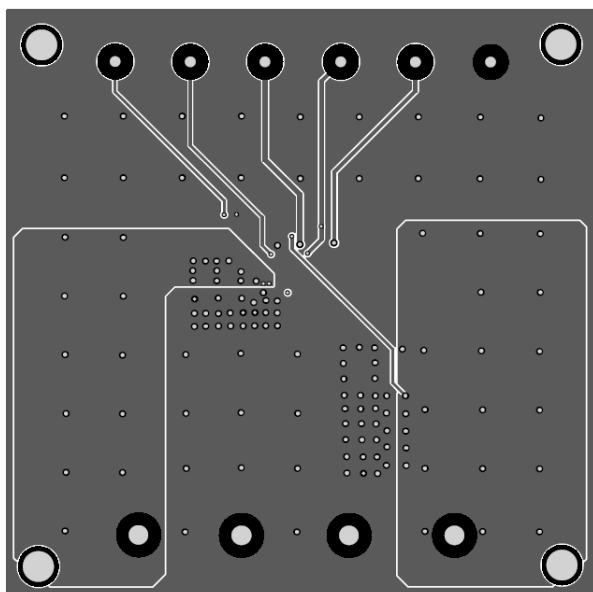
Figure 3: Inner Layer 2
