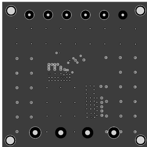
Figure 2: Inner Layer 1
