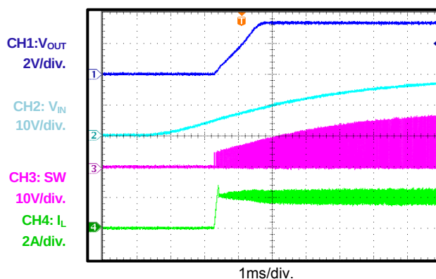
Startup through Input Voltage I_{OUT} = 2A
