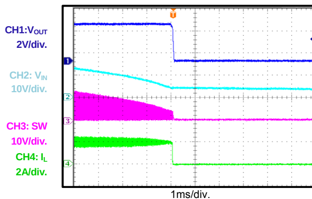
Shutdown through Input Voltage I_{OUT} = 2A
