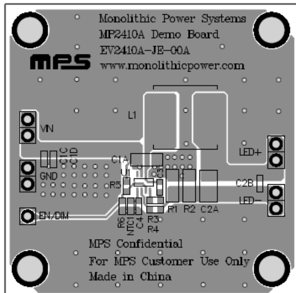
Figure 2 - Top Layer
