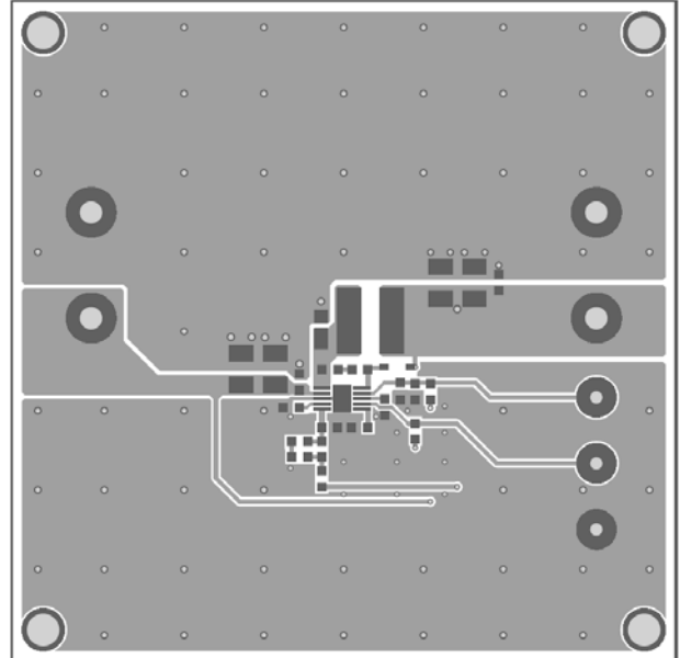
Figure 2 – Top Layer
